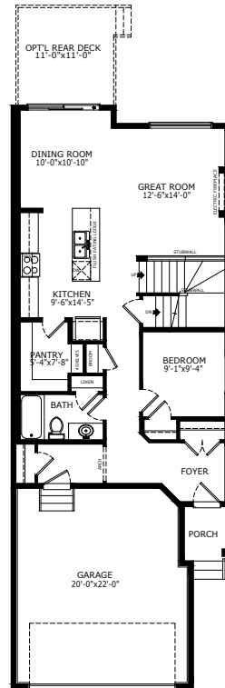
OPTIONAL FULL BATH WITH BEDROOM
